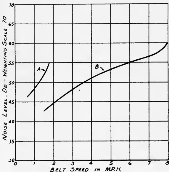
FIG. 2. Noise measurements of treadmill.
